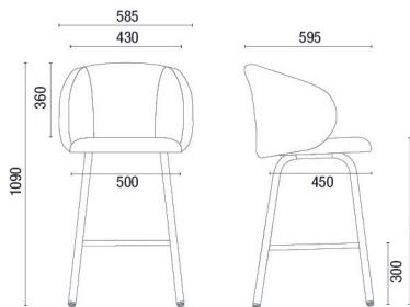
36.706 Fixed Wood Legs
