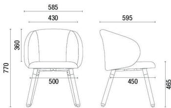
36.706 Fixed Wood Legs
