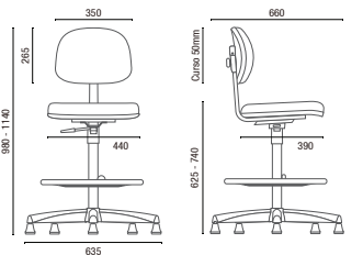
4022 BG Secretaria Stool
