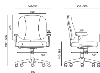
4003 Director Giratoria Extra
