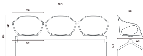
33110 Longarina
