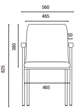
18006 Z Visitor Chair
