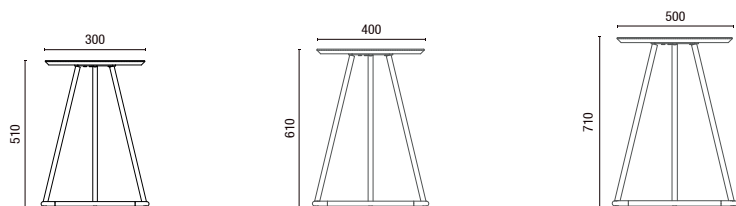
39.801 Mesa Lateral
